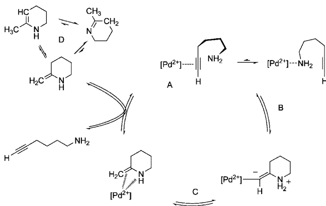
Scheme 59
