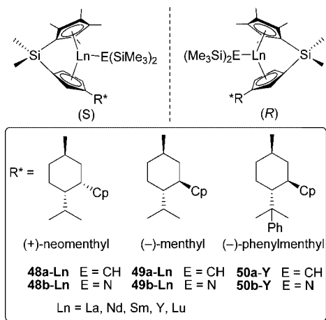
Figure 11. Chiral lanthanocene precatalysts for asymmetric hydroamination.
