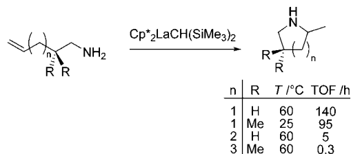
Scheme 8. Lanthanocene-Catalyzed Hydroamination/Cyclization of Aminoalkynes 96
