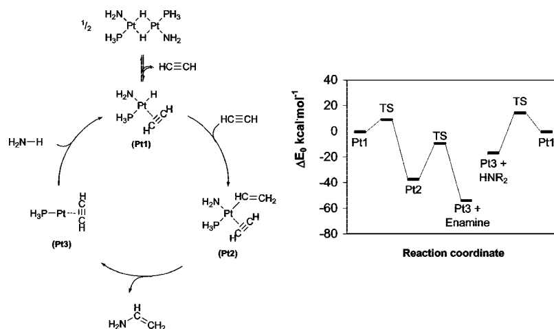
Figure 30. Reaction intermediates and energy diagram calculated for the platinum-catalyzed hydroamination of ethyne with ammonia.
