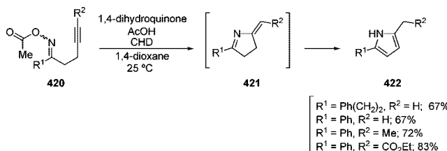
Scheme 173
