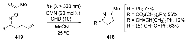
Scheme 172
